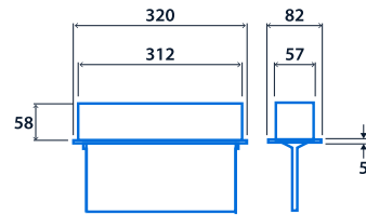
Semi Recessed
