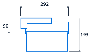
Cantilever Mounting
