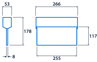
Ceiling Mounting
